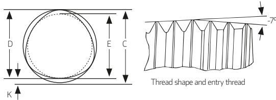
Taptite trilobular geometry
