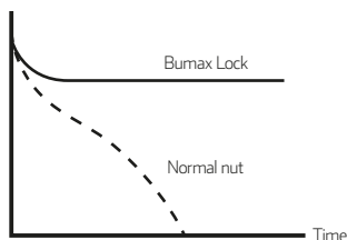
Fig 3. Residual stress
