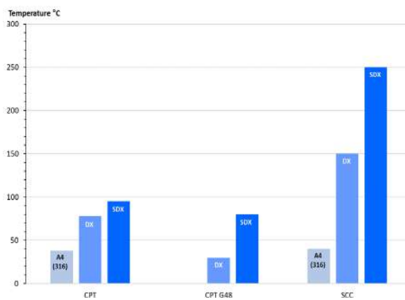
Figure 3: Laboratory corrosion specimen testing results.
